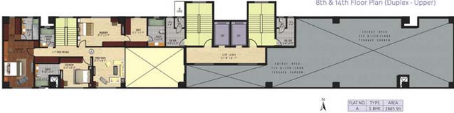
Block-B & C 8th & 14th Floor Plan (Duplex - Upper)
