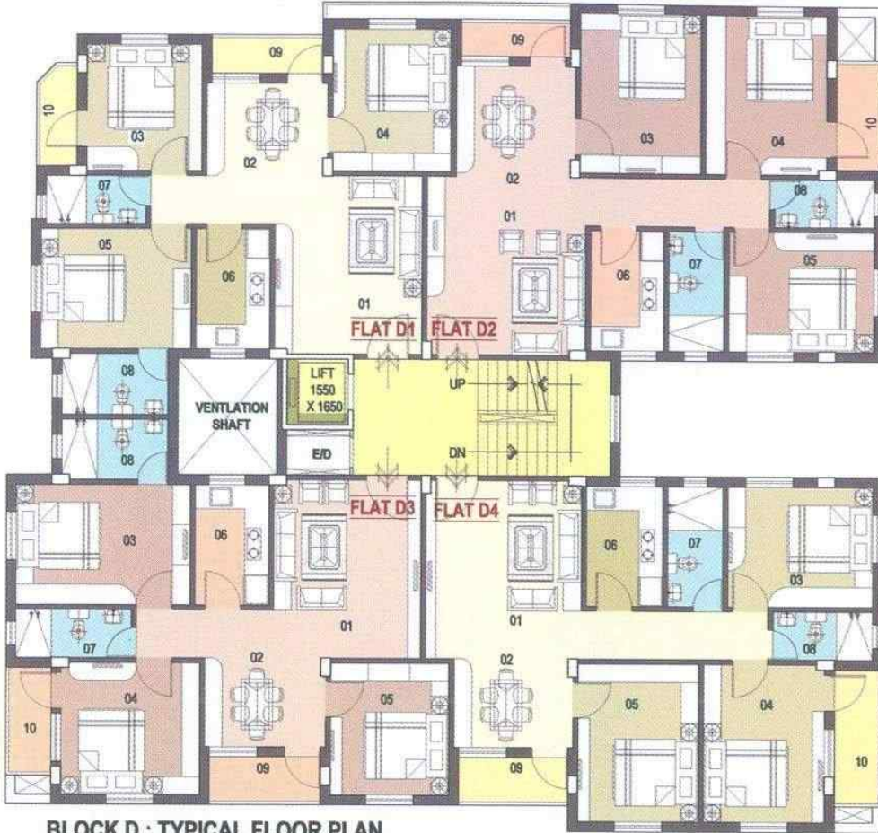
BLOCK D : TYPICAL FLOOR PLAN
