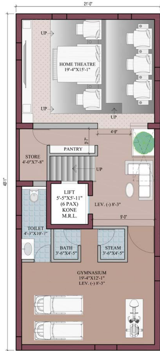
BASEMENT PLAN
