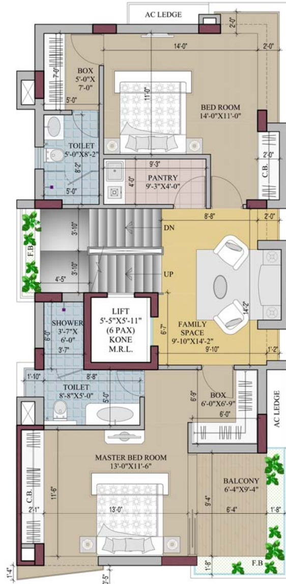
TYPICAL FL. PLAN (2ND. TO 4TH.)
